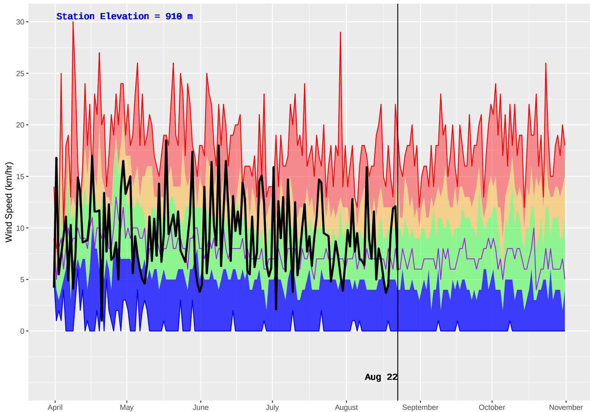
NAZKO (211) : Historical (1981–2016) and Current (2018) Daily Wind Speed
