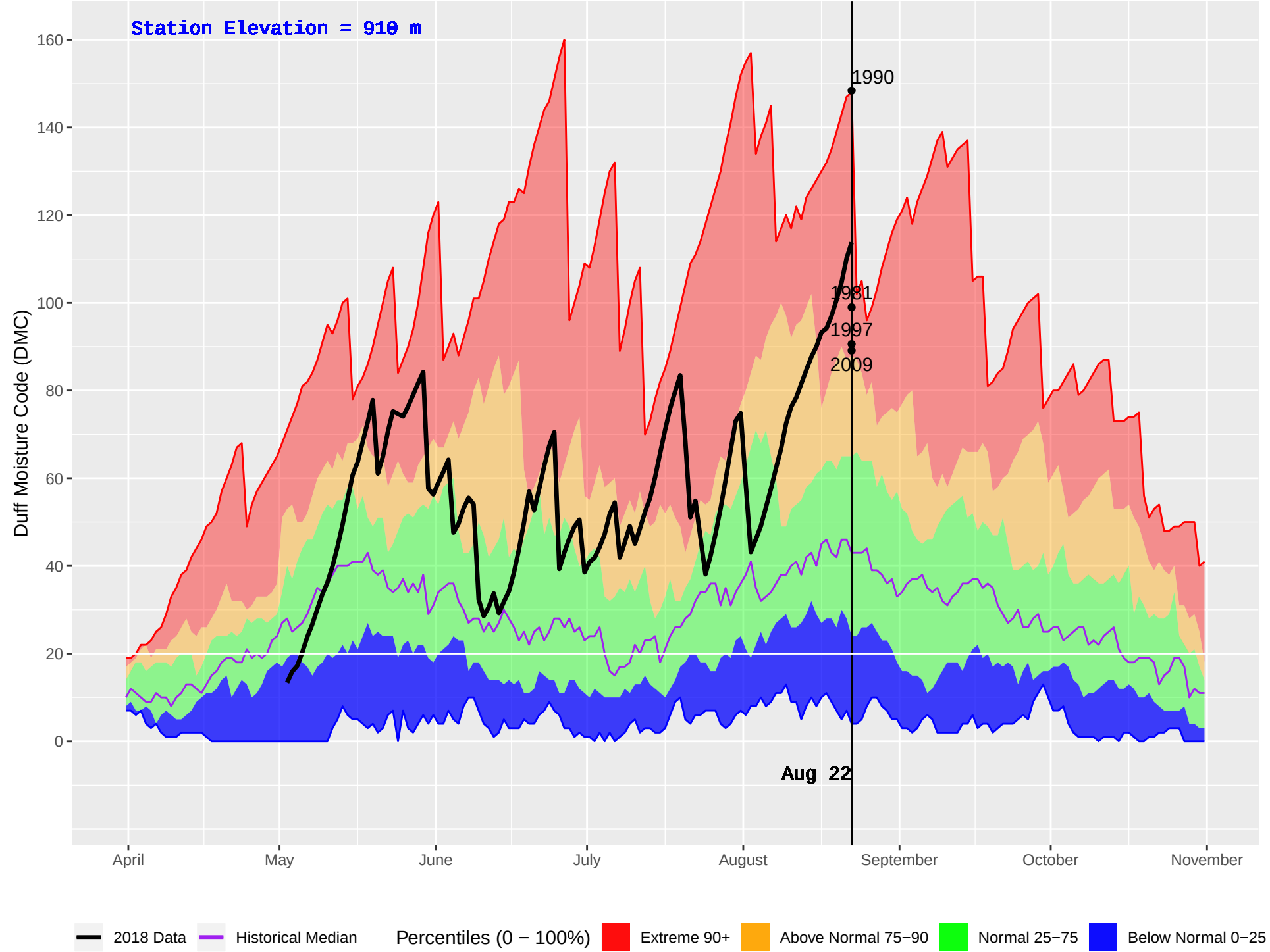
NAZKO (211) : Historical (1981–2016) and Current (2018) Daily Duff Moisture Code (DMC)
