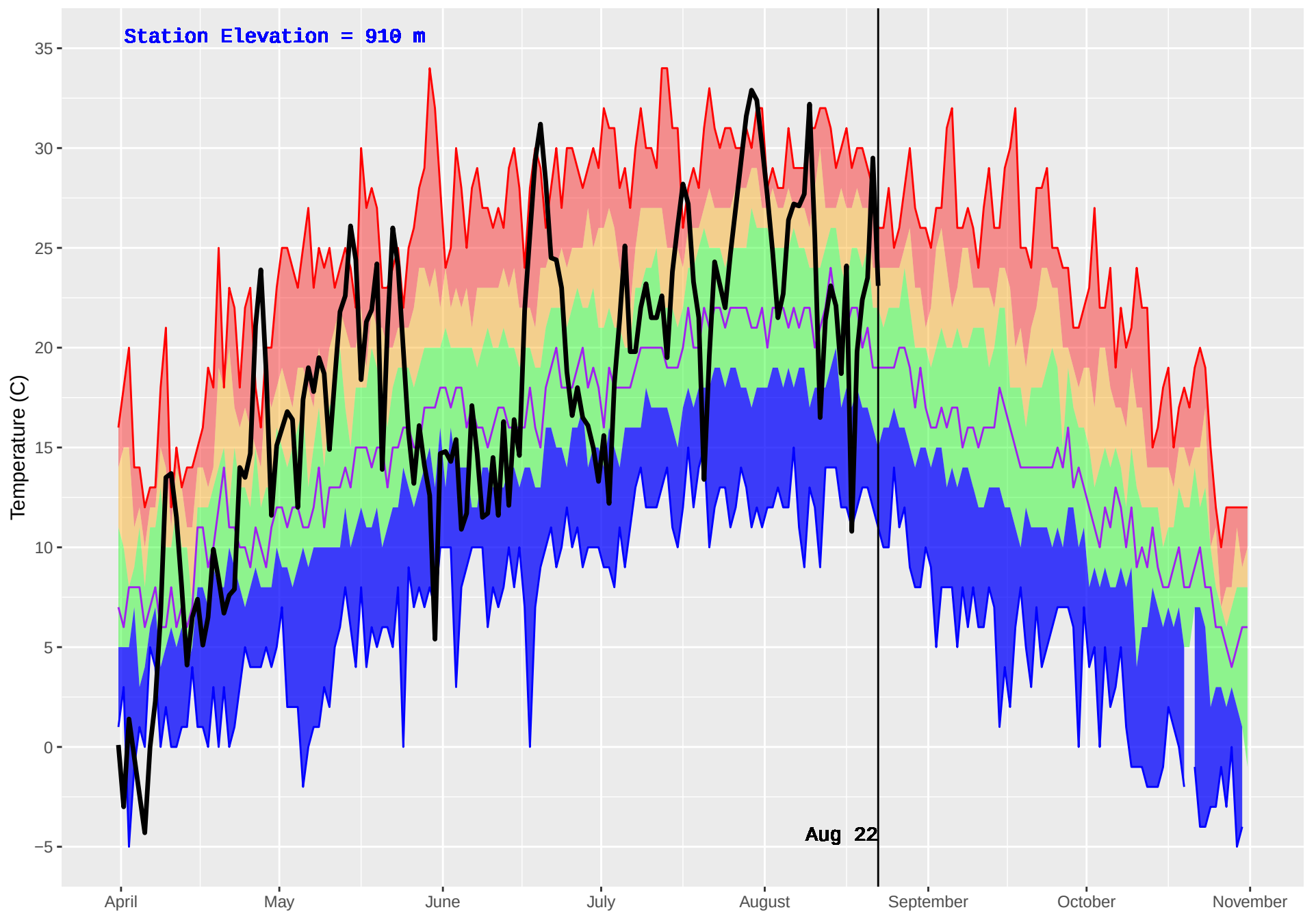
NAZKO (211) : Historical (1981–2016) and Current (2018) Daily Temperature
