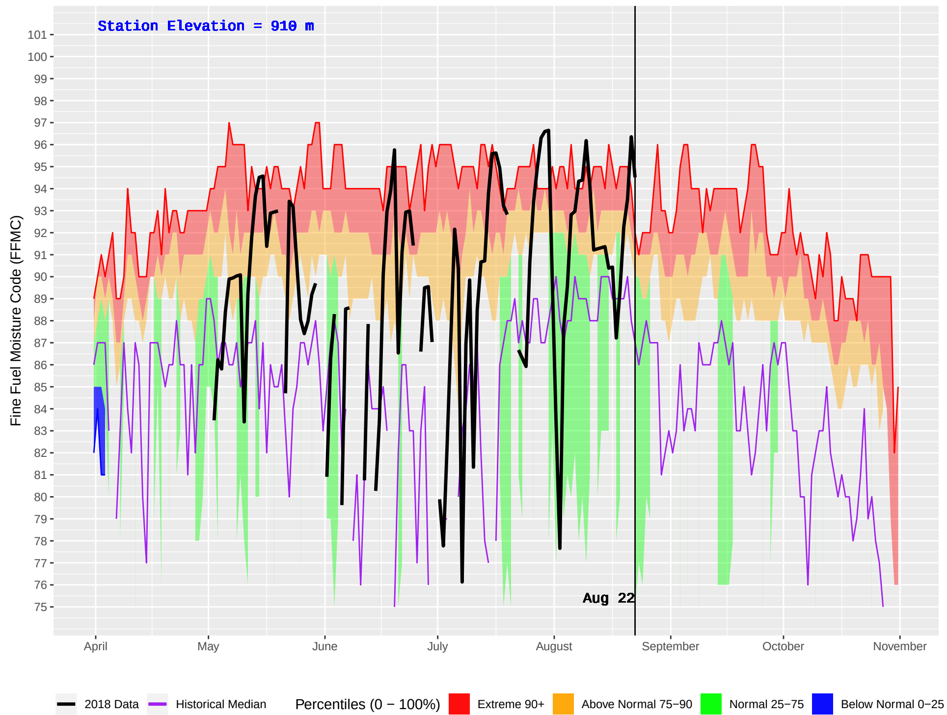
NAZKO (211) : Historical (1981–2016) and Current (2018) Daily Fine Fuel Moisture Code (FFMC)
