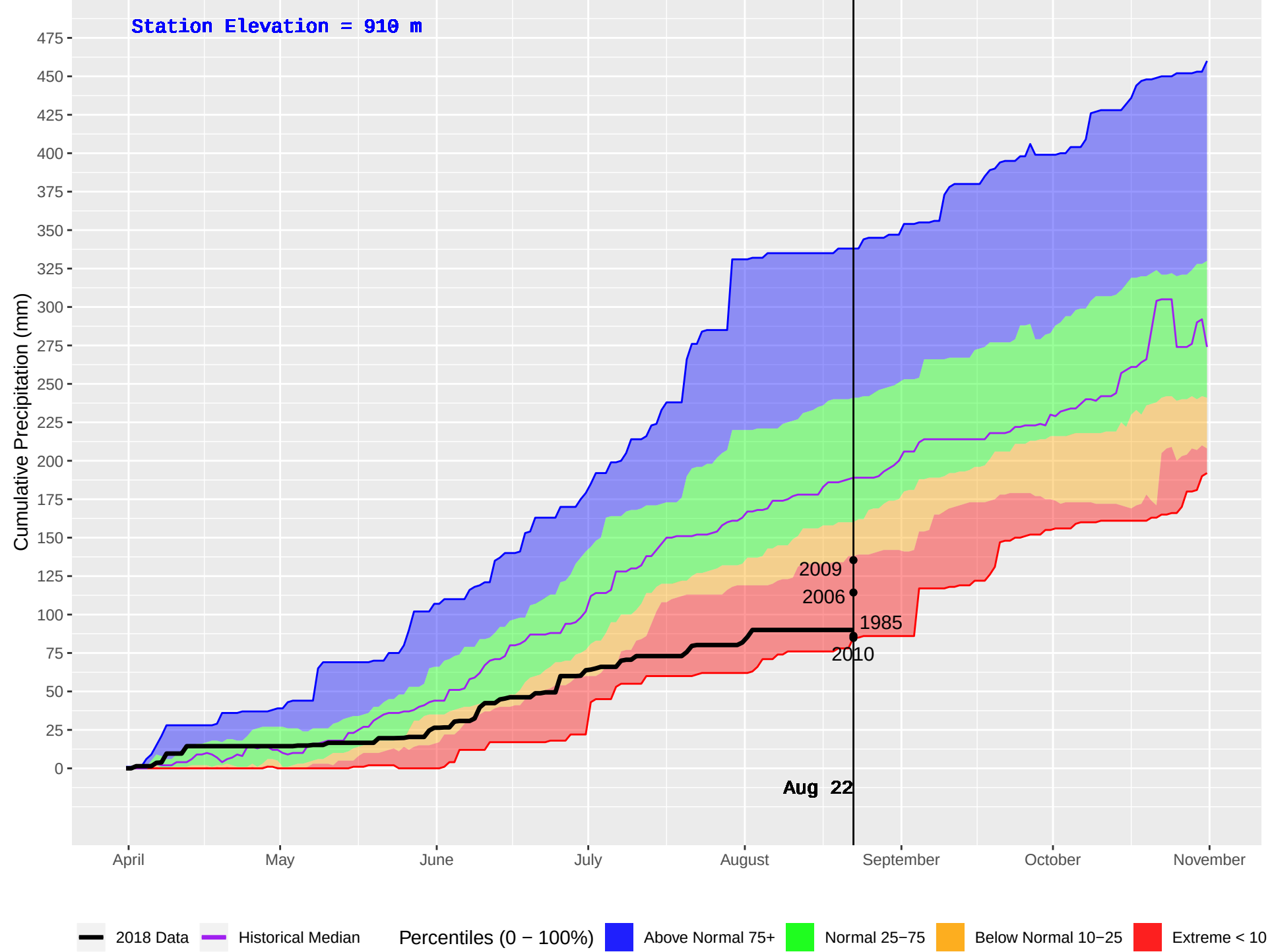
NAZKO (211) : Historical (1981–2016) and Current (2018) Daily Cumulative Precipitation
