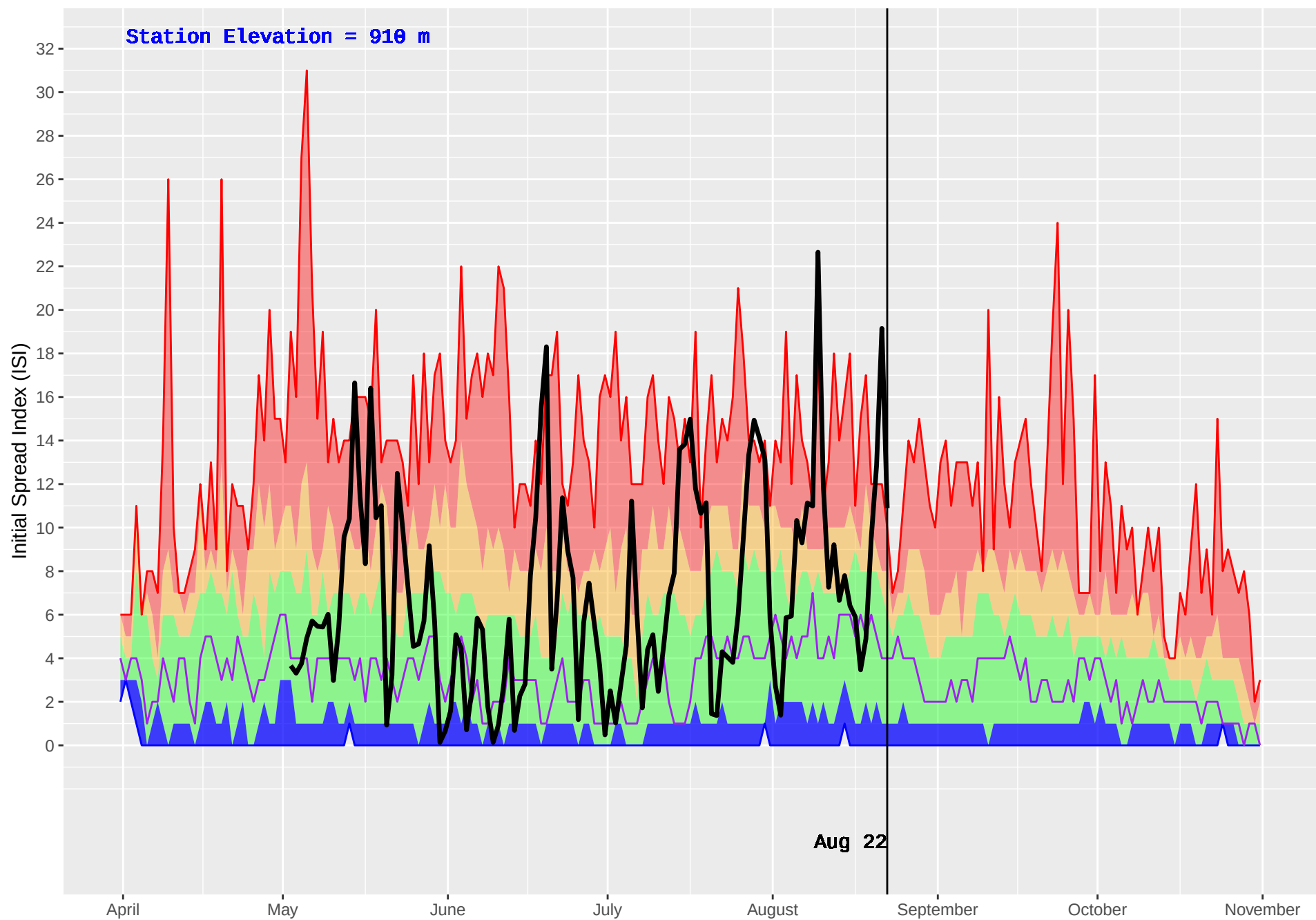
NAZKO (211) : Historical (1981–2016) and Current (2018) Daily Initial Spread Index (ISI)
