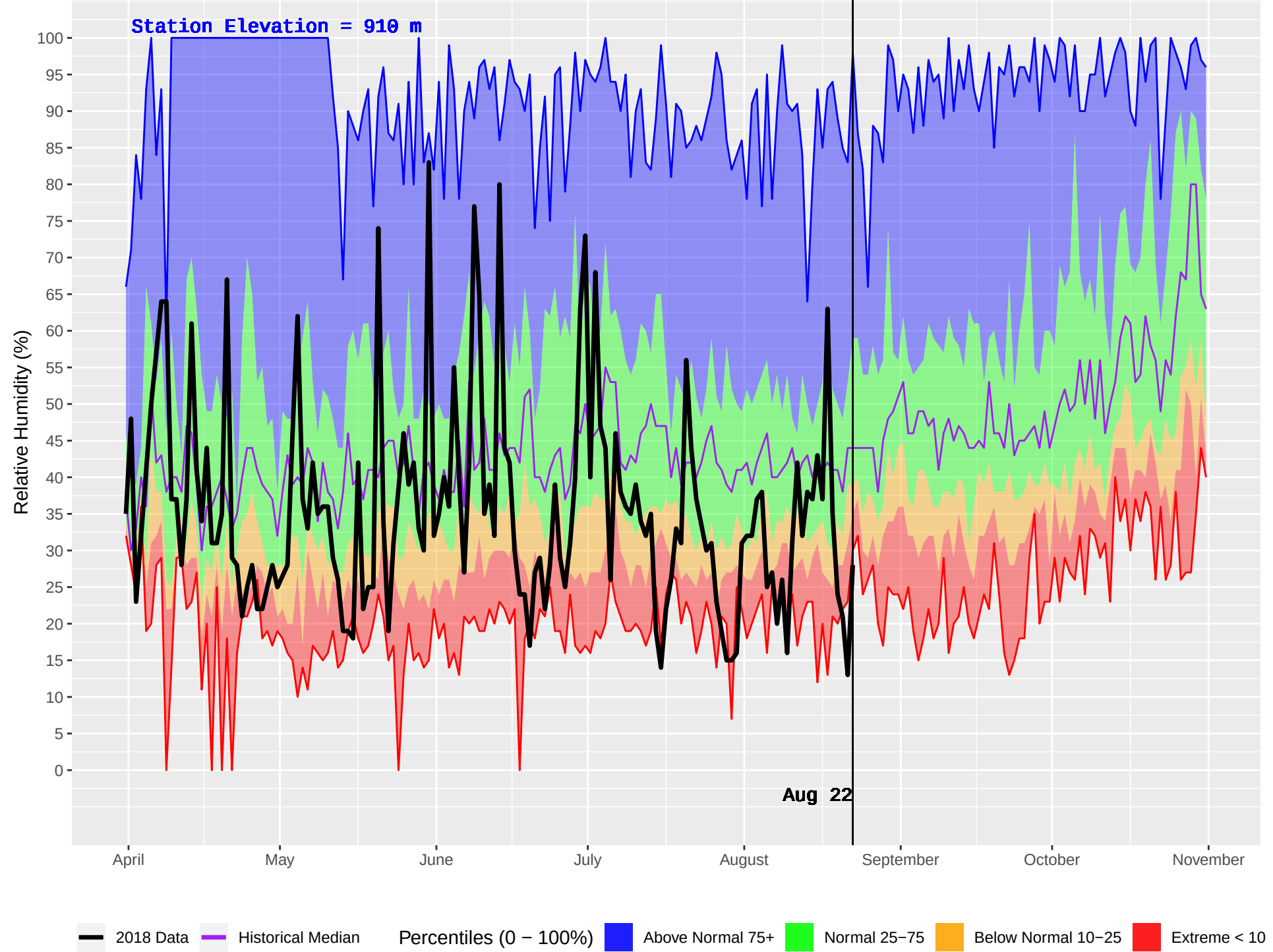
NAZKO (211) : Historical (1981–2016) and Current (2018) Daily Relative Humidity
