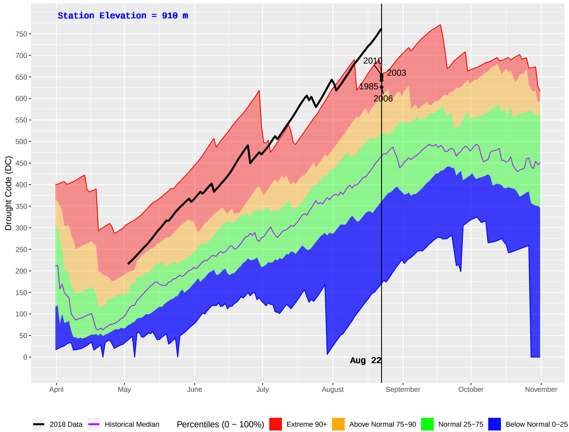
NAZKO (211) : Historical (1981–2016) and Current (2018) Daily Drought Code (DC)
