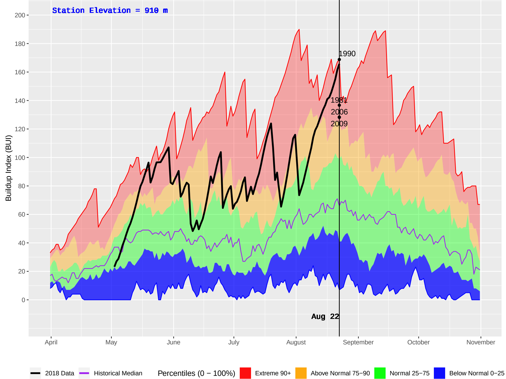
NAZKO (211) : Historical (1981–2016) and Current (2018) Daily Buildup Index (BUI)
